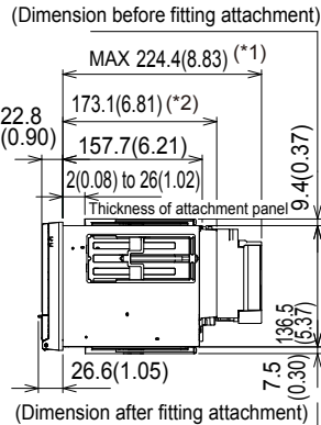
Side-by-Side Mounting (horizontally)
