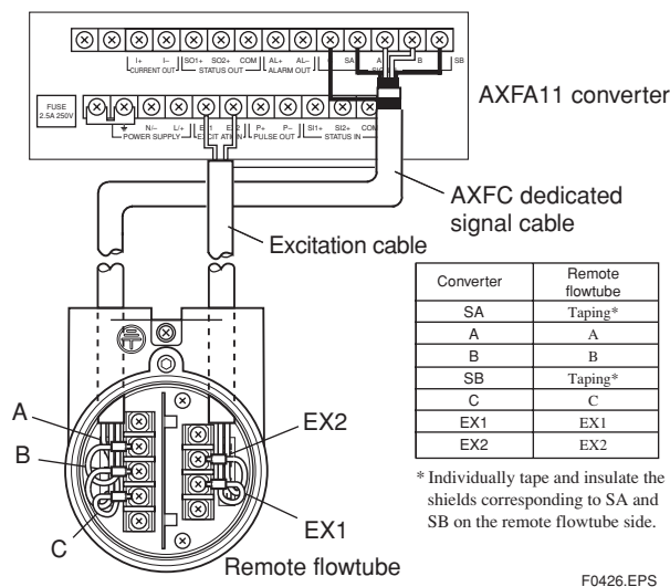
Figure 4.2.13 Wiring Diagram
