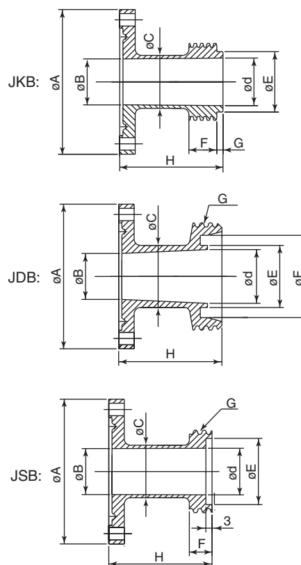
Adapters for union connection
