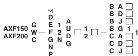
Integral Flowmeter
