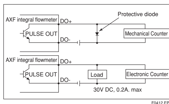
Figure 4.1.11 Pulse Output Connection
