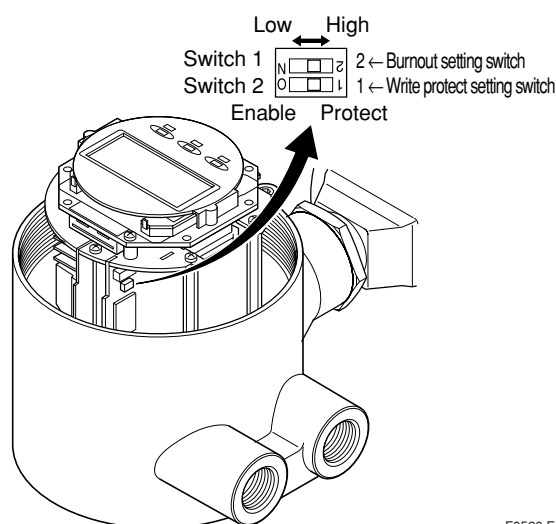
Figure 5.5.1 Switch Configuration
