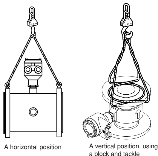
Figure 3.2.1 Lifting Flowmeter
