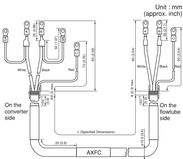
Figure 4.2.2 Treatment of Dedicated Signal Cables
