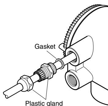
Figure 4.2.6 Plastic Gland (Optional code EP)
