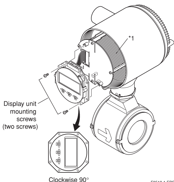
Figure 5.4.2 Changing the Display Unit Direction 90 Degrees
