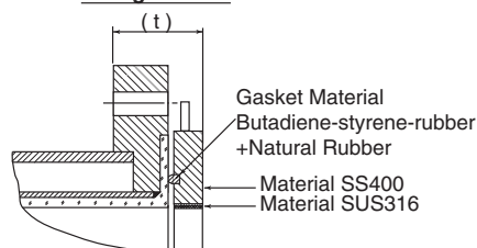
Flange Detail
