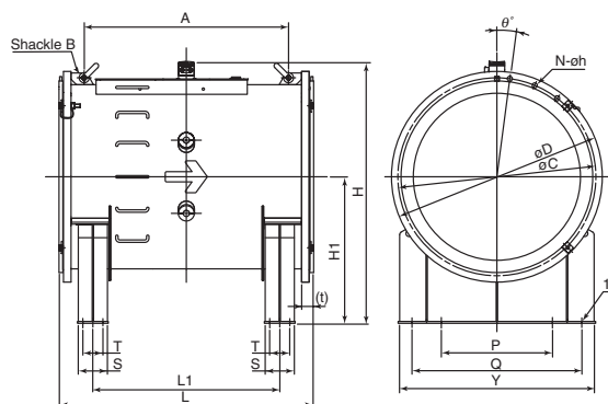
Flange Detail
