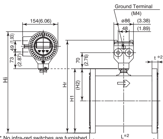
Integral Flowmeter
