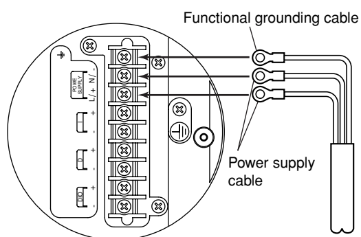
Figure 4.1.7 Electric Cable Wiring
