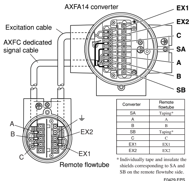
Figure 4.2.16 Wiring Diagram
