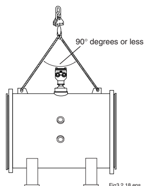
Figure 3.3.6 Lifting Flowtube
