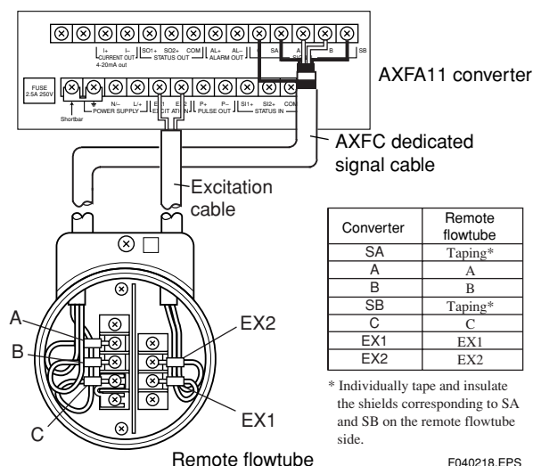
Figure 4.2.18 Wiring Diagram
