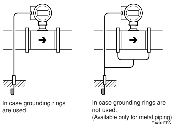
Figure 4.1.9 Grounding
