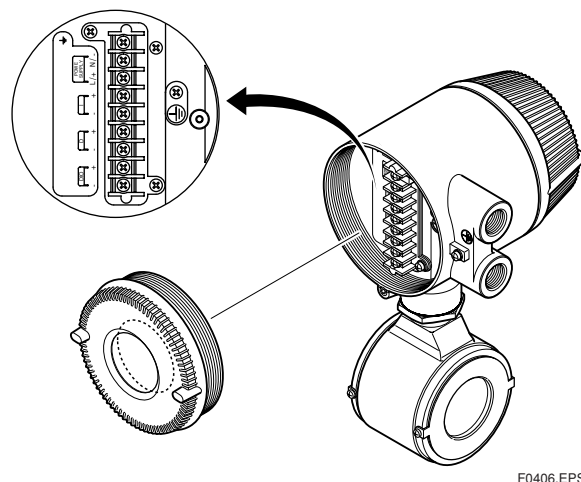
Figure 4.1.6 Terminal Configuration
